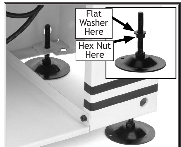
Figure 14. Installed feet.
